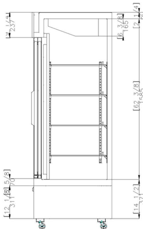
SIDE VIEW
